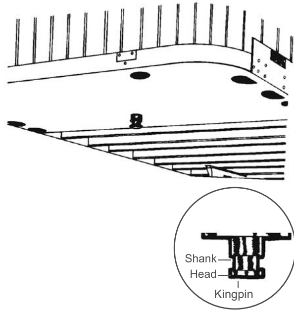
Figure 6-7: Trailer Kingpin
